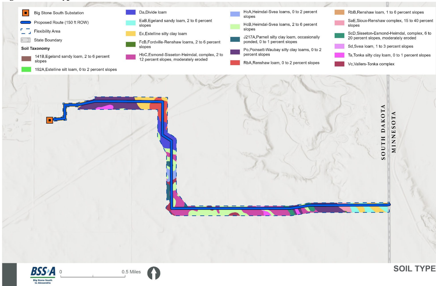
Figure 13. Soil types
