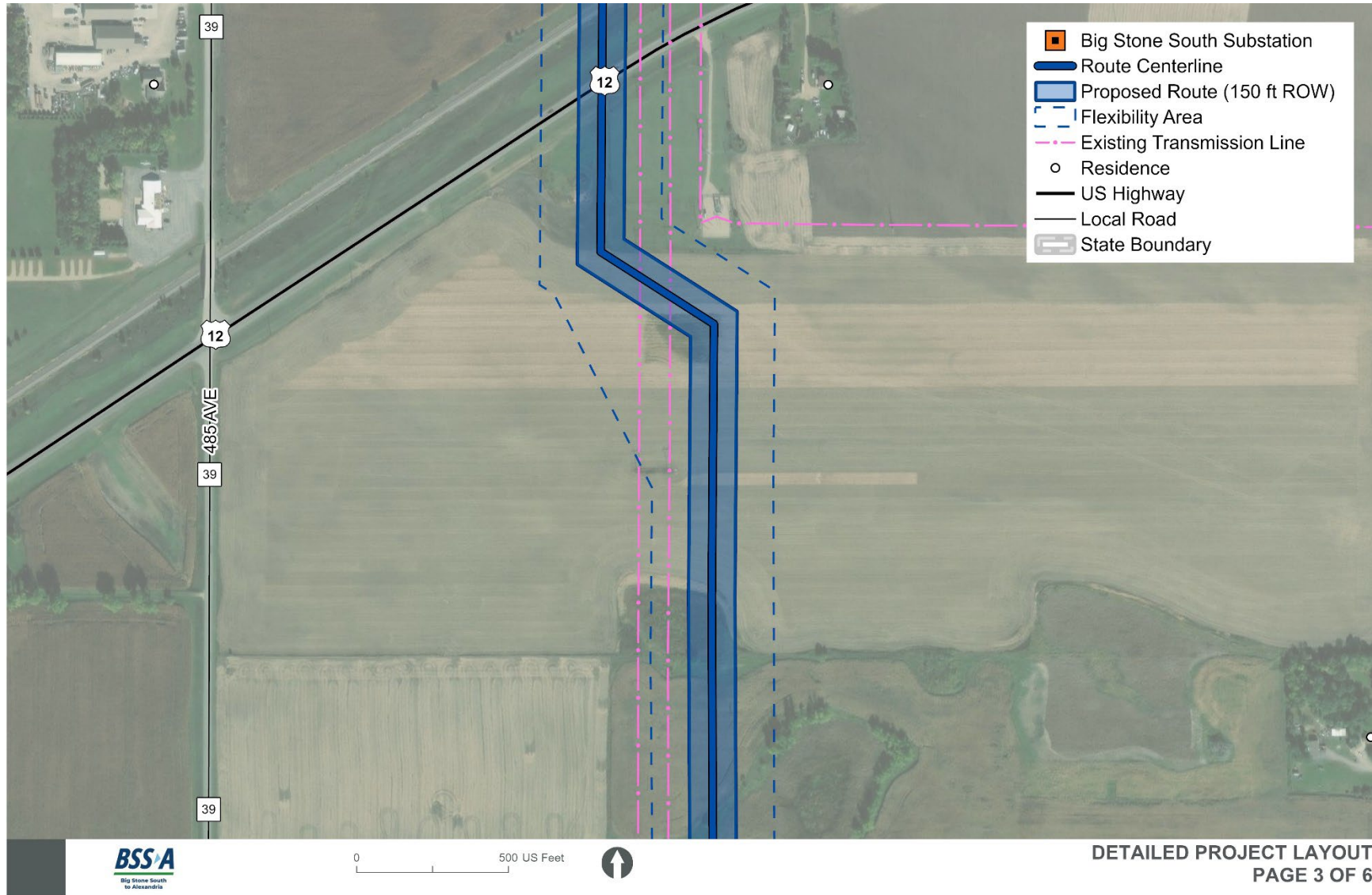
Figure 4c. Detailed Project layout
