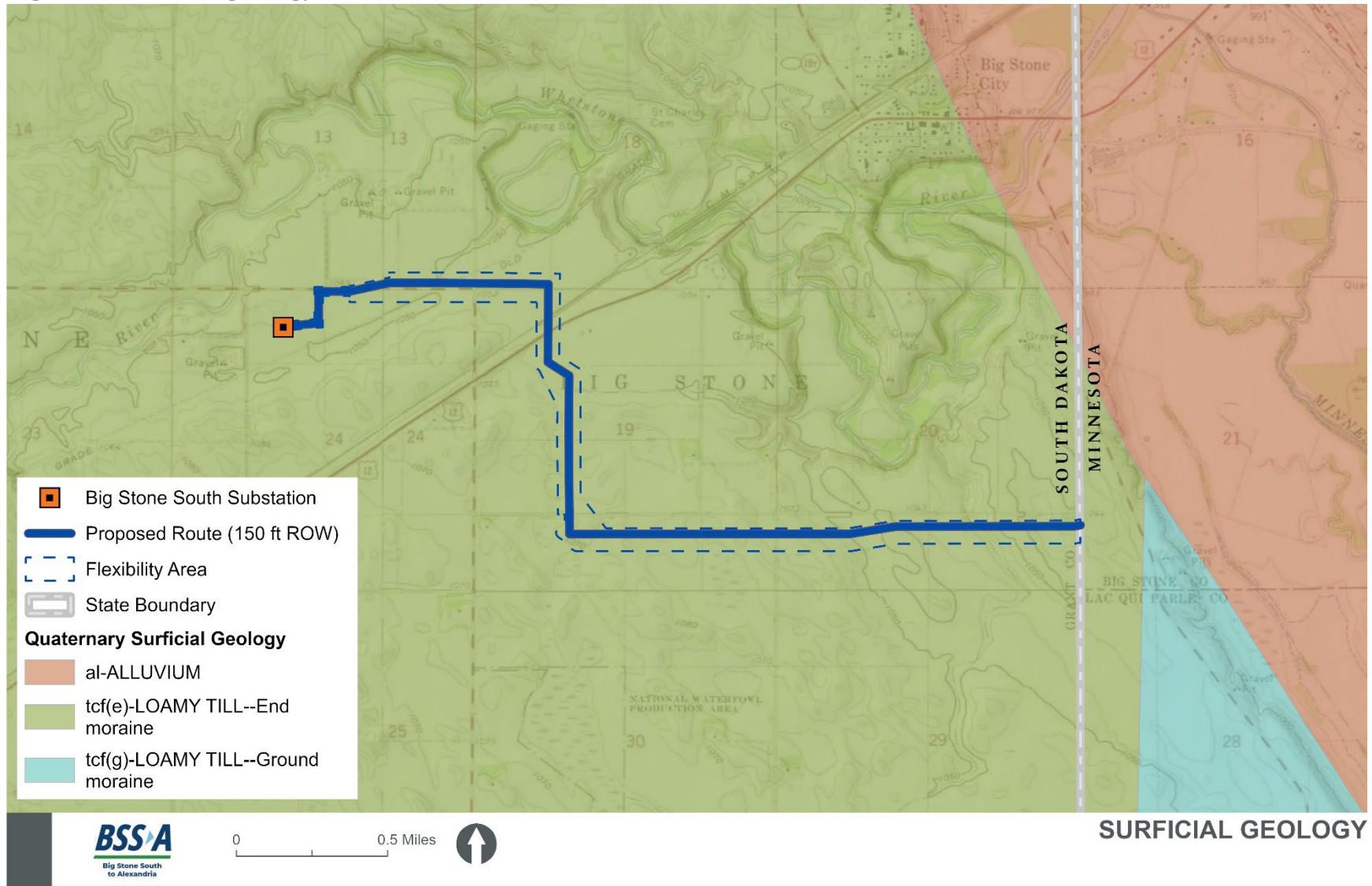
Figure 9. Surficial geology
